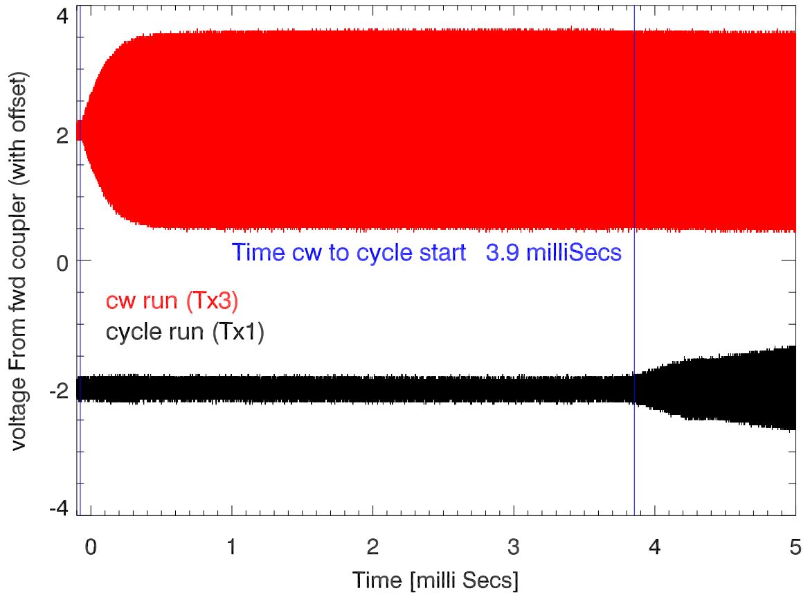
26jun17 time CW,Cycle output (at coupler) rise times.
