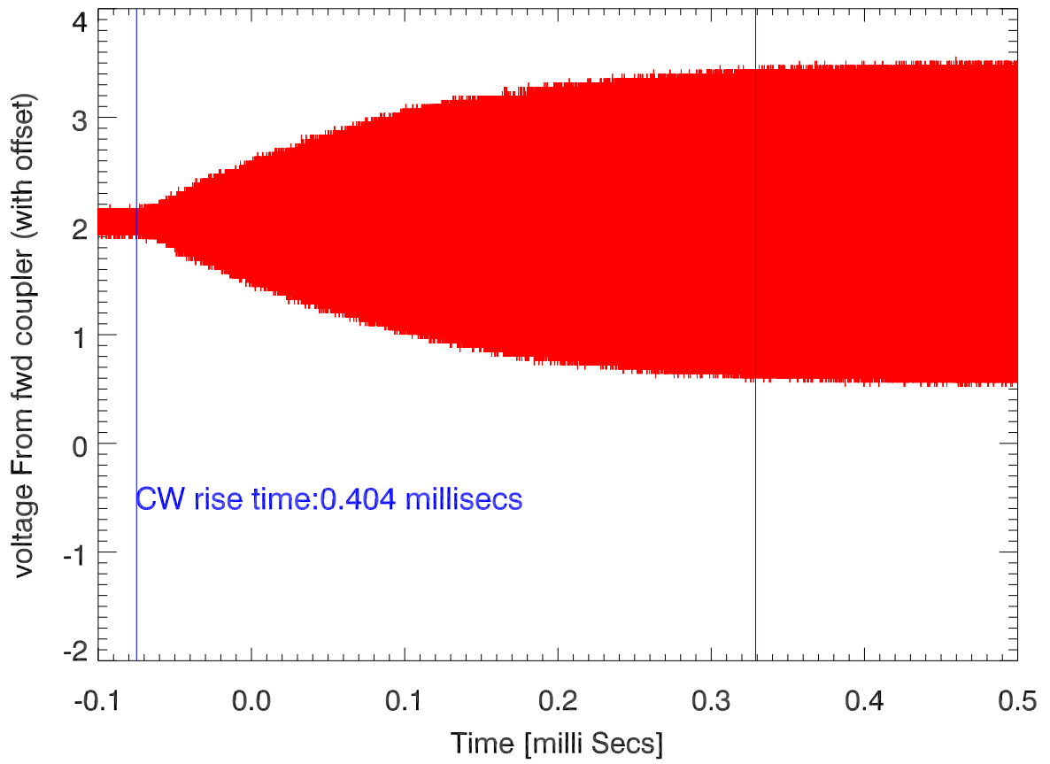
26jun17 CW rise time (from output coupler)
