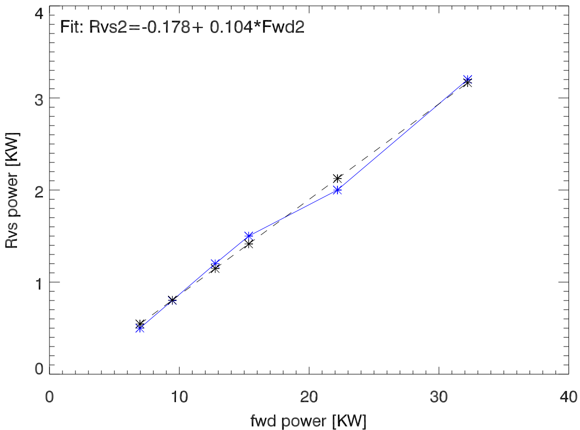
05oct16 8MHz Tx2 Alone: Fit RvsPower vs FwdPower
