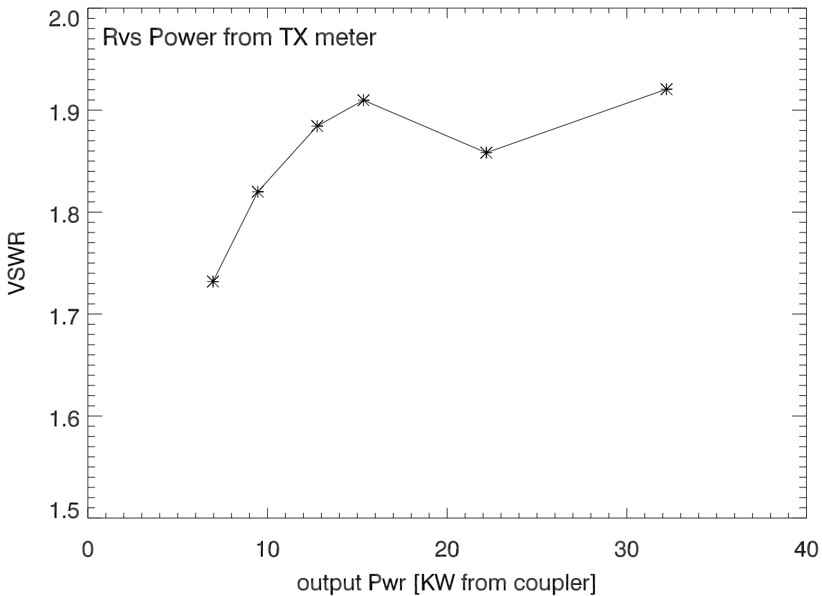
Tx2 VSWR vs output pwr. (Only Tx2)
