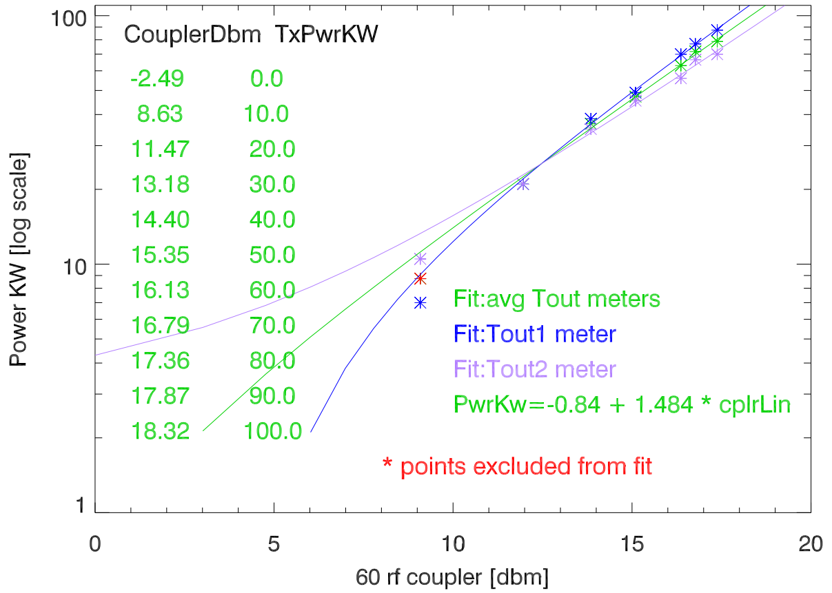
tx2 output power vs rf Coupler
