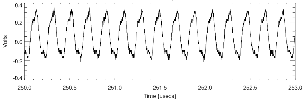
Driver output
