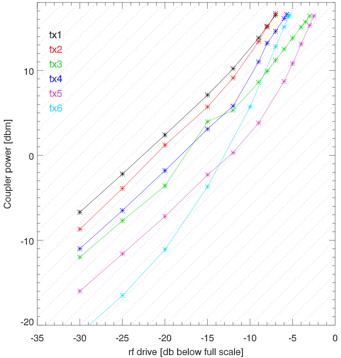
29oct15 Output pwr vs rf drive (dbm vs dbf). on antenna
