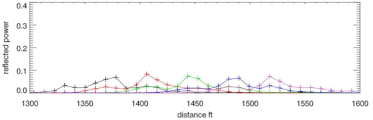
Blowup near short. uncorrected phase
