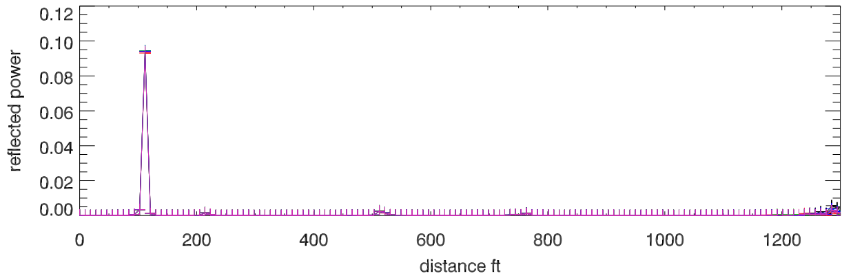
Reflected power vs distance. uncorrected phase. 0..1300 ft
