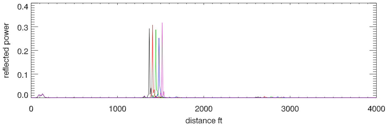
Reflected power vs distance. Corrected phase. 0-4000 ft
