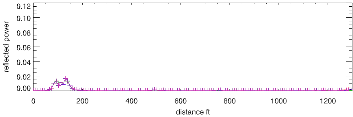
Reflected power vs distance. Corrected phase. 0..1300 ft
