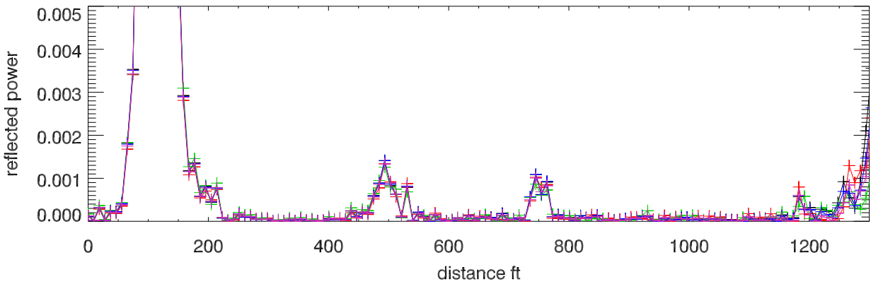
Corrected phase (blowup 0..1300 ft)
