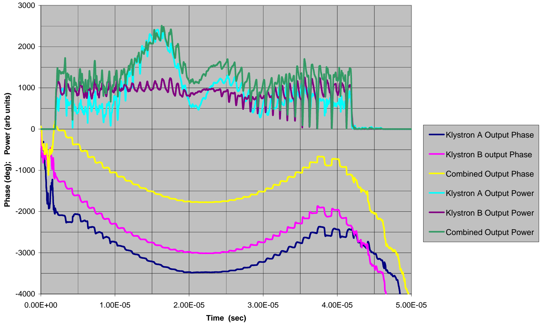
430 TX Power & Phase vs Time
