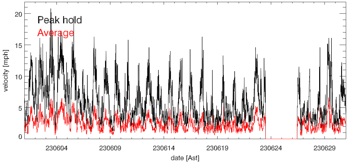
jun23 Avg & Peak velocities vs date (over 15.0 minutes)
