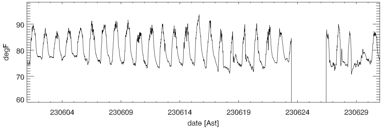
jun23 Temp vs date (averaged over 15.0 minutes)
