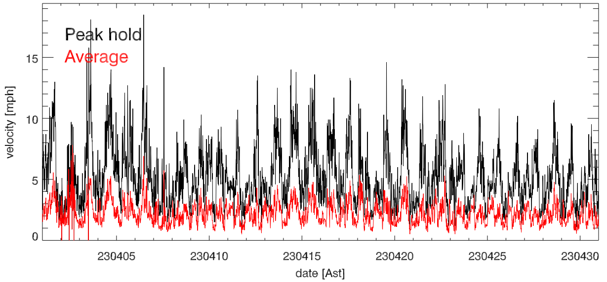
apr23 Avg & Peak velocities vs date (over 15.0 minutes)
