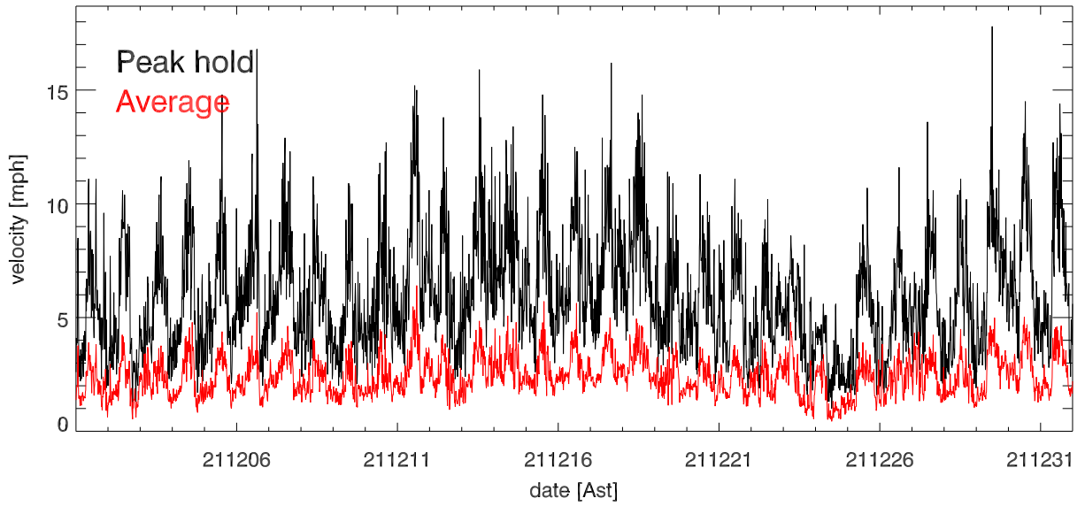
dec21 Avg & Peak velocities vs date (over 15.0 minutes)
