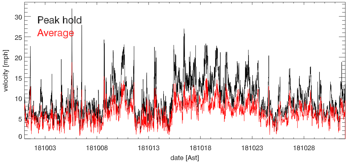
oct18 Avg & Peak velocities vs date (over 15.0 minutes)
