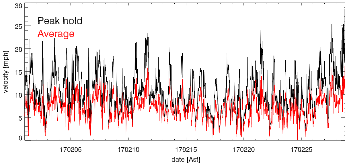
feb17 Avg & Peak velocities vs date (over 15.0 minutes)
