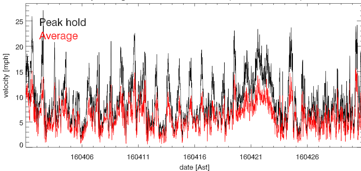
apr16 Avg & Peak velocities vs date (over 15.0 minutes)
