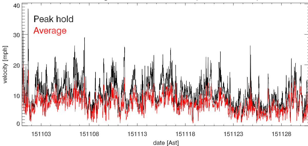
nov15 Avg & Peak velocities vs date (over 15.0 minutes)
