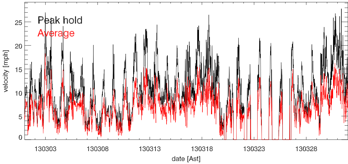
mar13 Avg & Peak velocities vs date (over 15.0 minutes)
