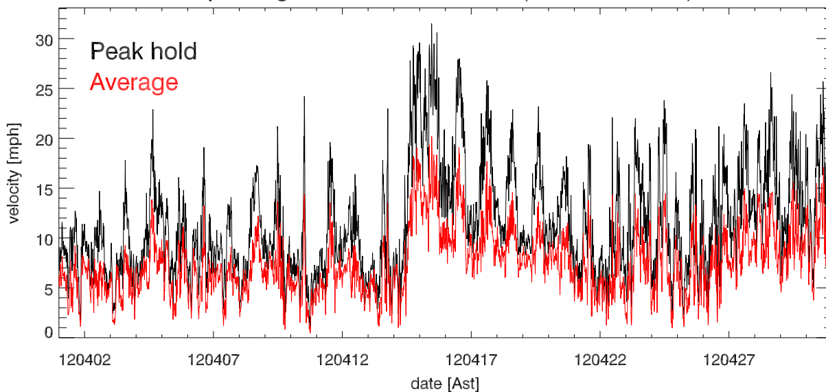
apr12 Avg & Peak velocities vs date (over 15.0 minutes)
