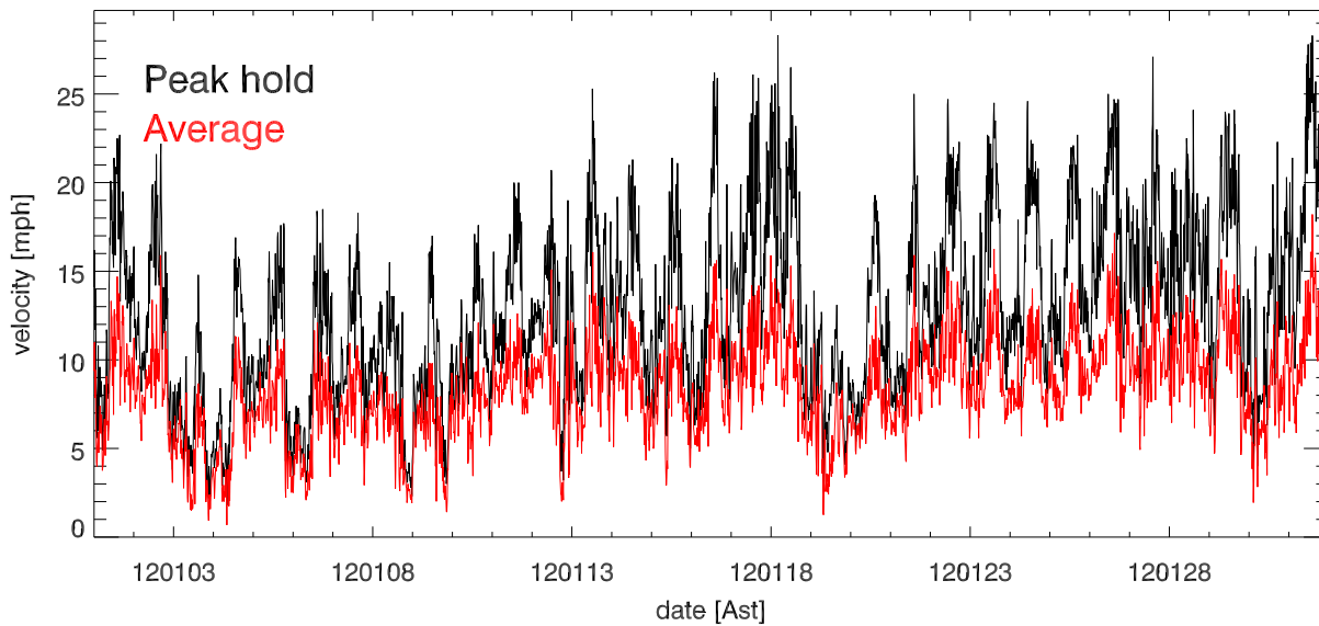
jan12 Avg & Peak velocities vs date (over 15.0 minutes)
