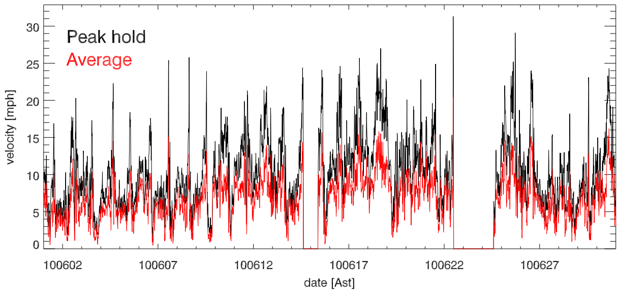
jun10 Avg & Peak velocities vs date (over 15.0 minutes)
