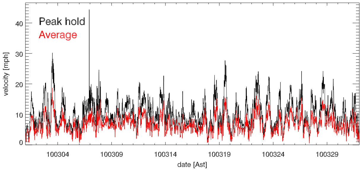
mar10 Avg & Peak velocities vs date (over 15.0 minutes)
