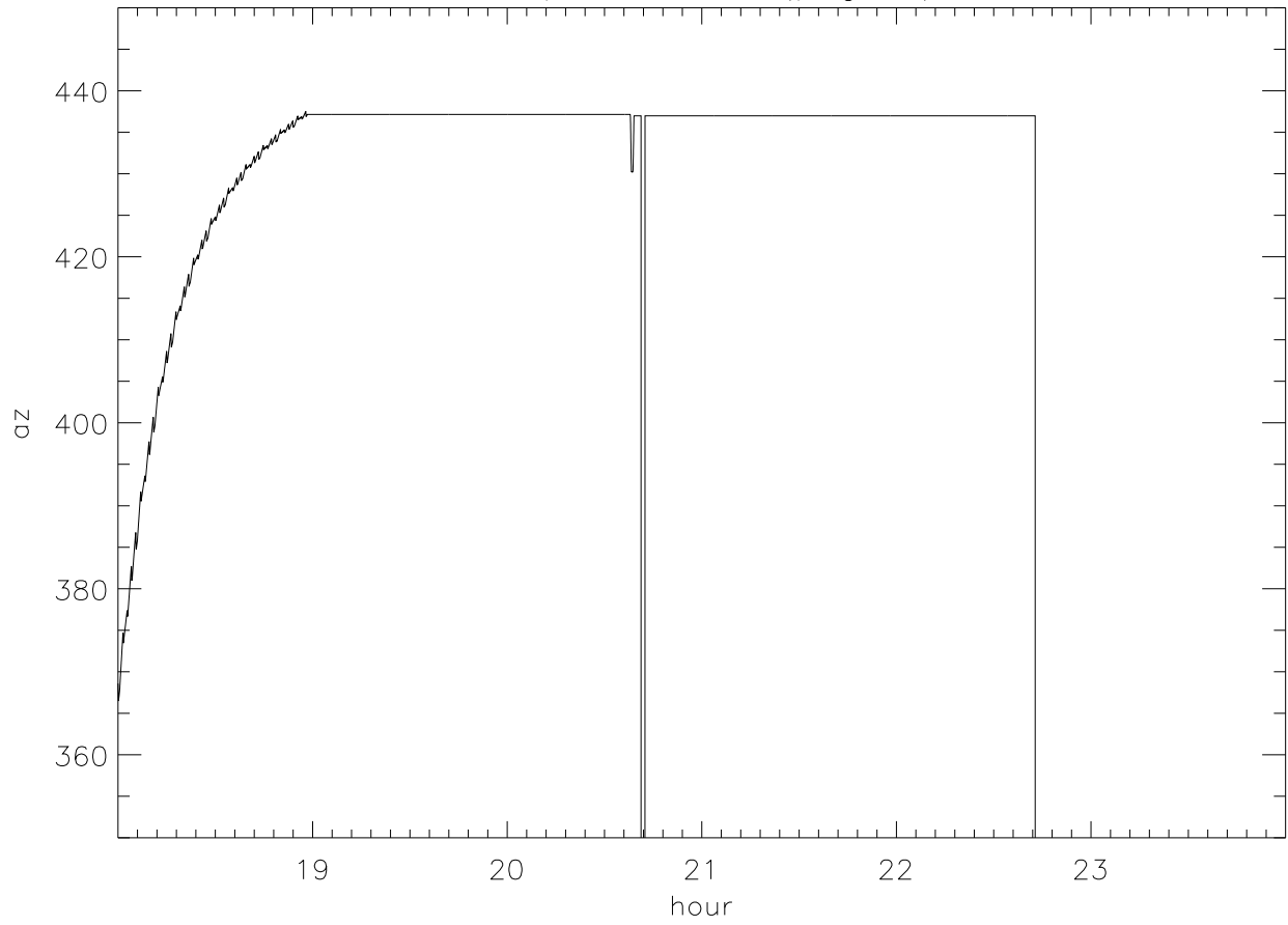
az encoder difference vs hour
