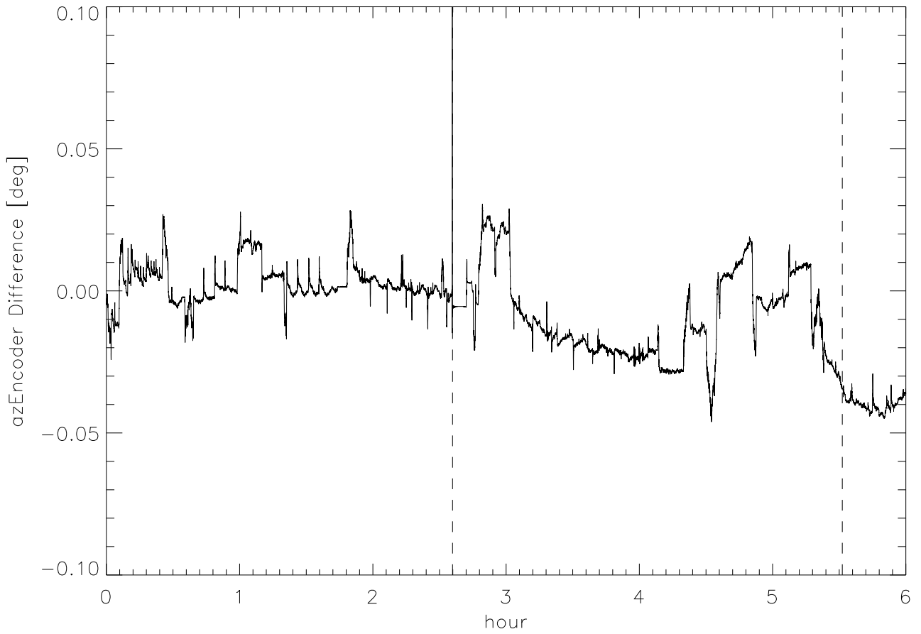
az encoder difference vs hour
