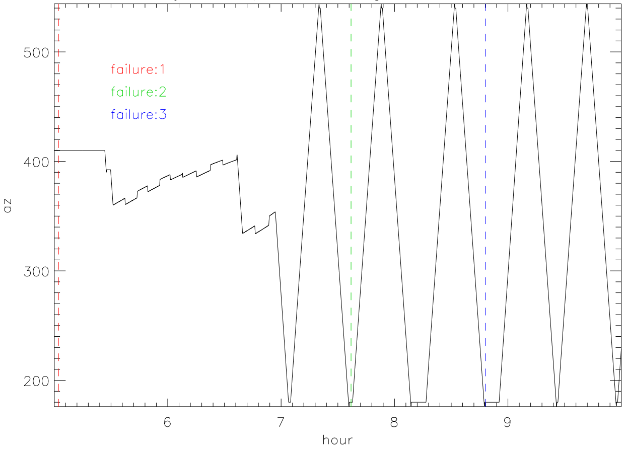
31jan10 azposition during motion failures
