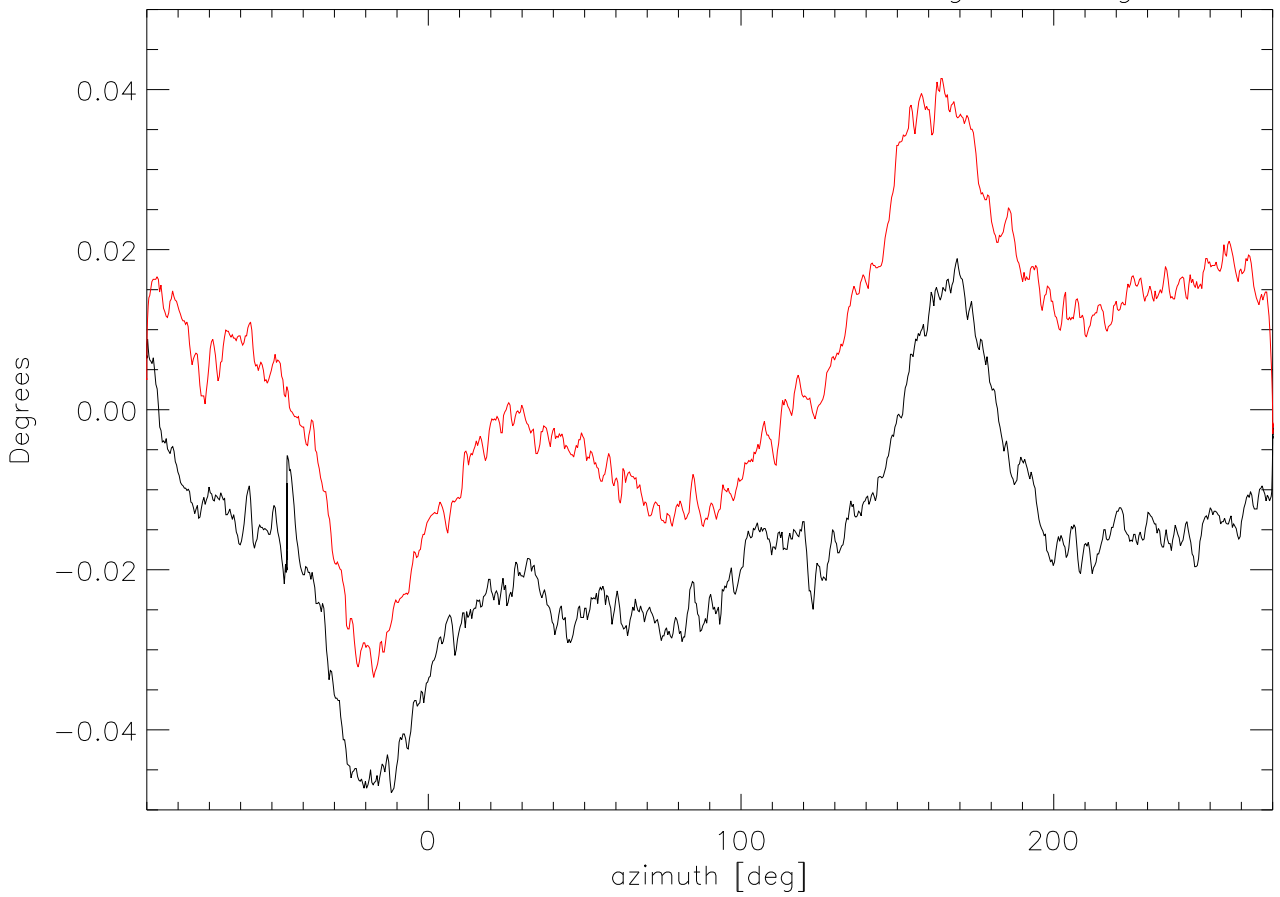
08mar06 az encoder difference during az swing
