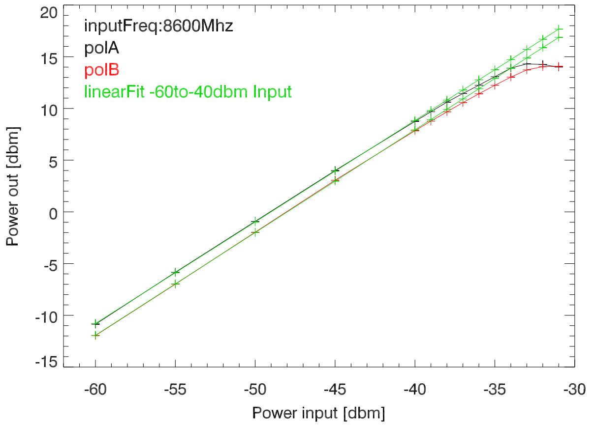
19nov21 measure linearity of udc synth chassis
