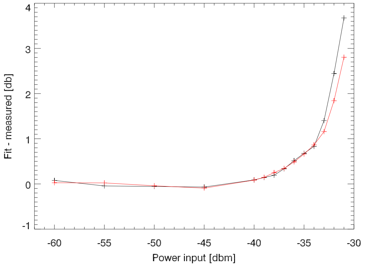
Linear fit - measured output power
