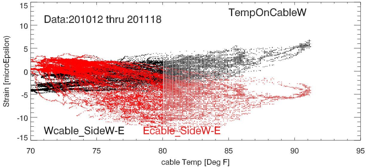
StrainDif (Side1 - Side2) vs cable temp. BackStay Tower 12
