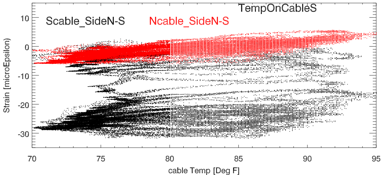
StrainDif (Side1 - Side2) vs cable temp. BackStay Tower 8
