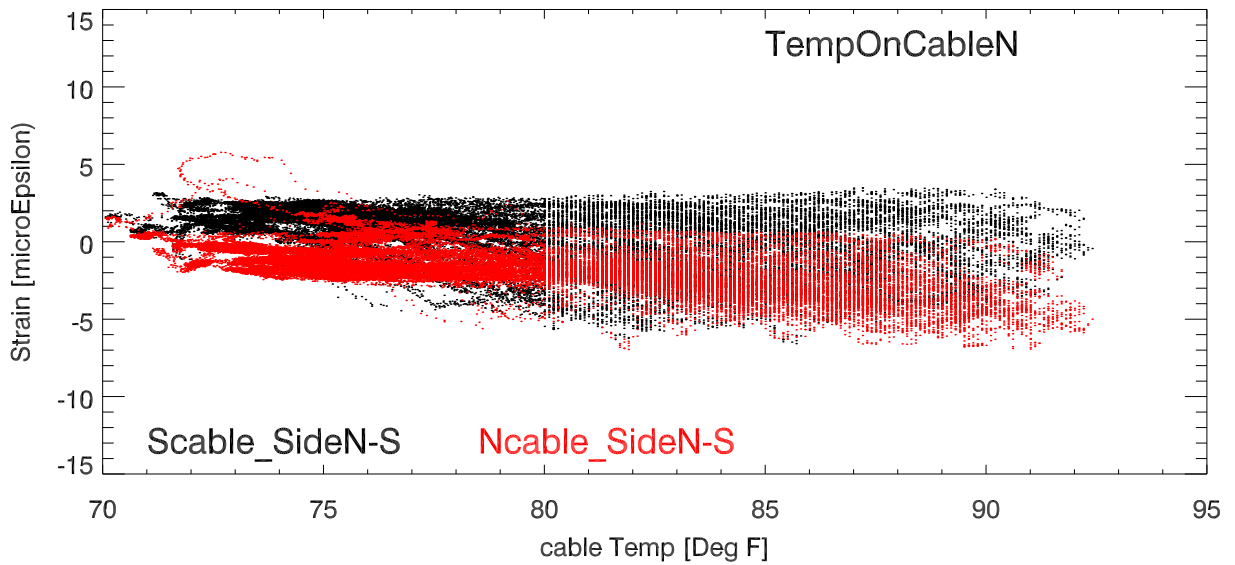
StrainDif (Side1 - Side2) vs cable temp. BackStay Tower 4
