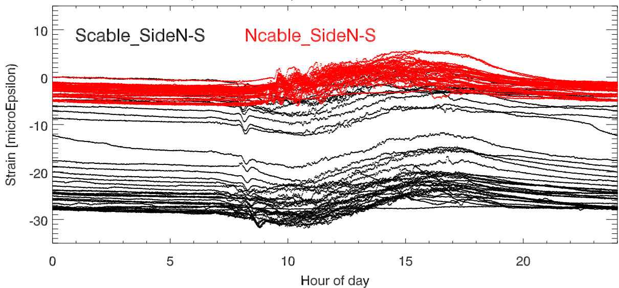
StrainDif (Side1 - Side2) vs Hour of day. BackStay Tower 8
