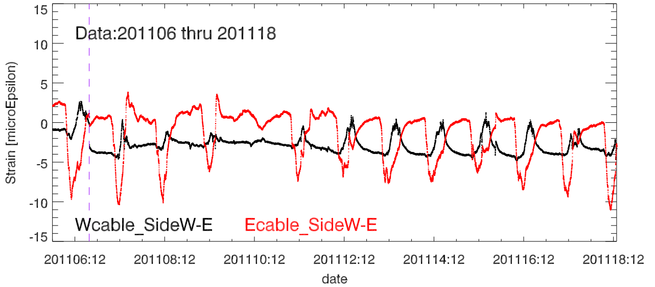
StrainDif (Side1 - Side2) vs date. BackStay Tower 12
