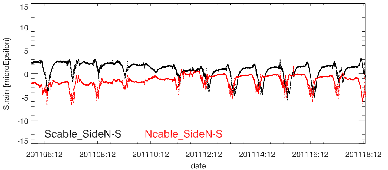
StrainDif (Side1 - Side2) vs date. BackStay Tower 4
