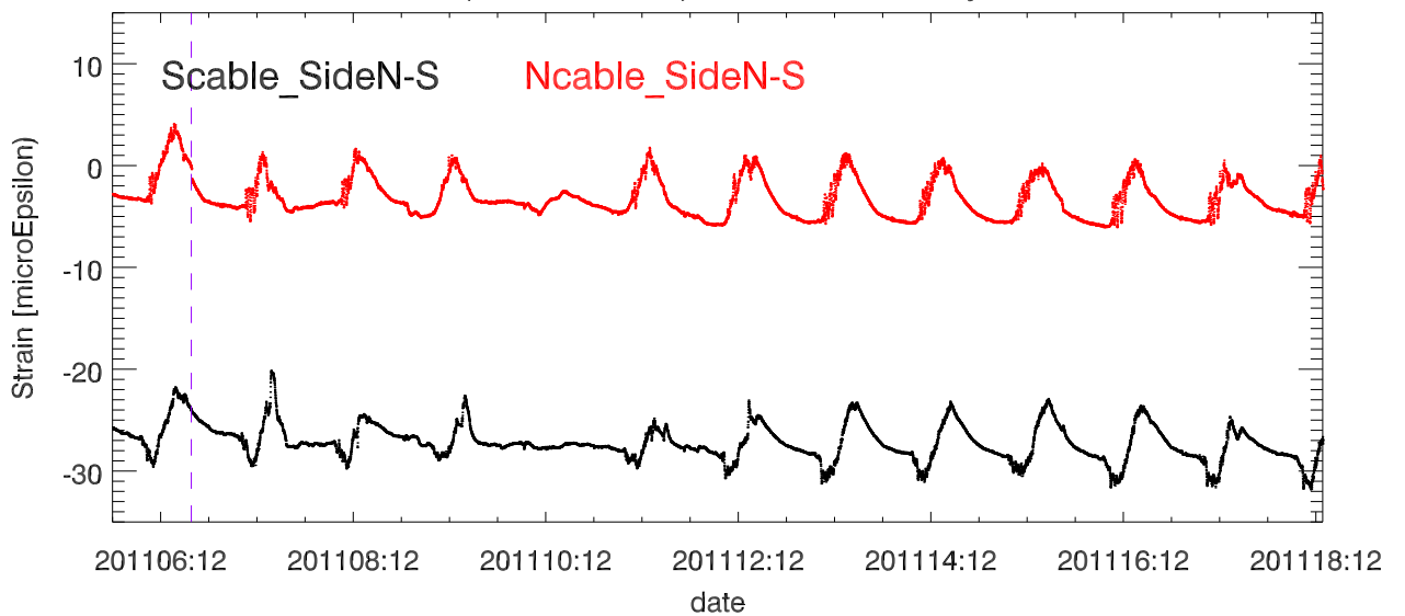
StrainDif (Side1 - Side2) vs date. BackStay Tower 8
