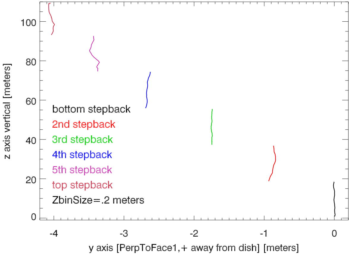
11nov20 T8 Face1. Avg Y motion vs height
