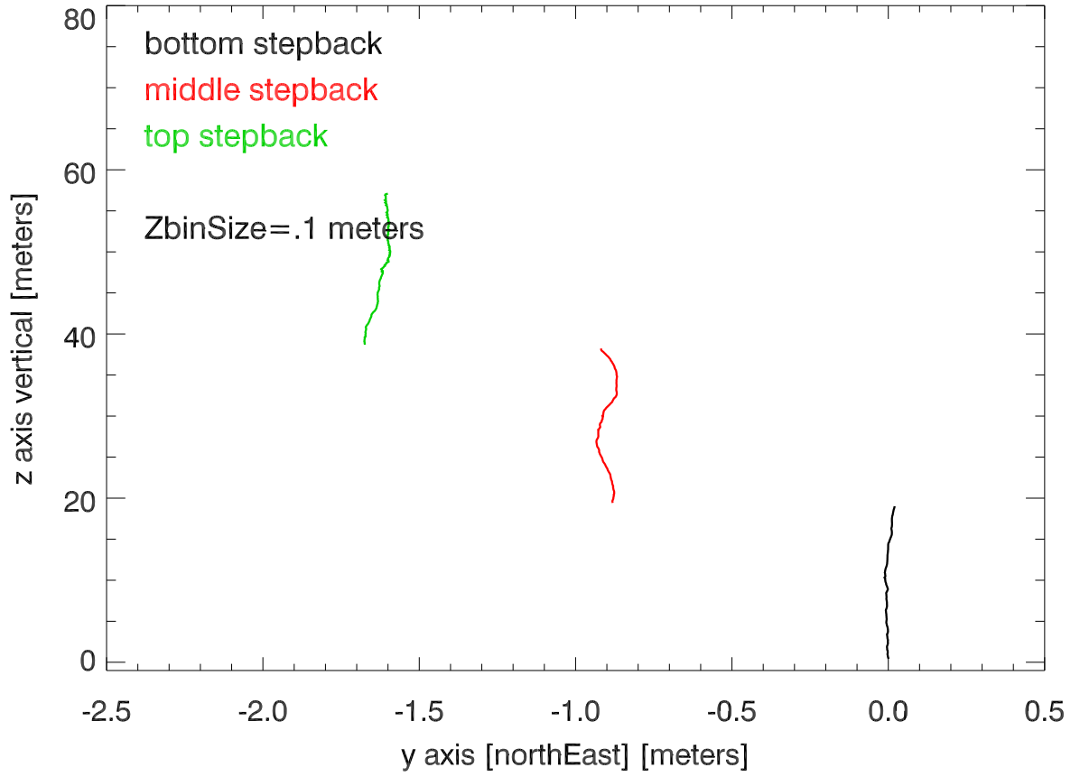
28dec20 T4 Face 2 (NE). Avg Y motion vs height
