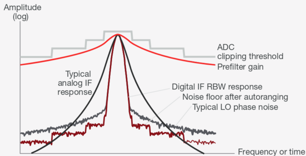
Figure 3-3. Autoranging keeps ADC noise close to the carrier and lower than LO noise or RBW filter response
