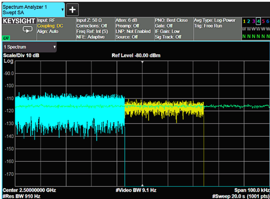
Figure 2-29. Smoothing effect of VBW-to-RBW ratios of 3:1, 1:10, and 1:100
