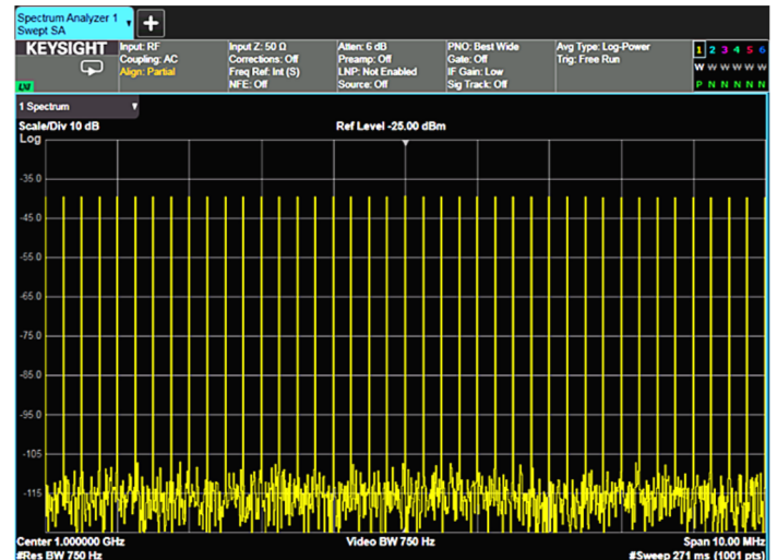
Figure 2-22b. The actual comb over a 10-MHz span using peak (positive) detection
