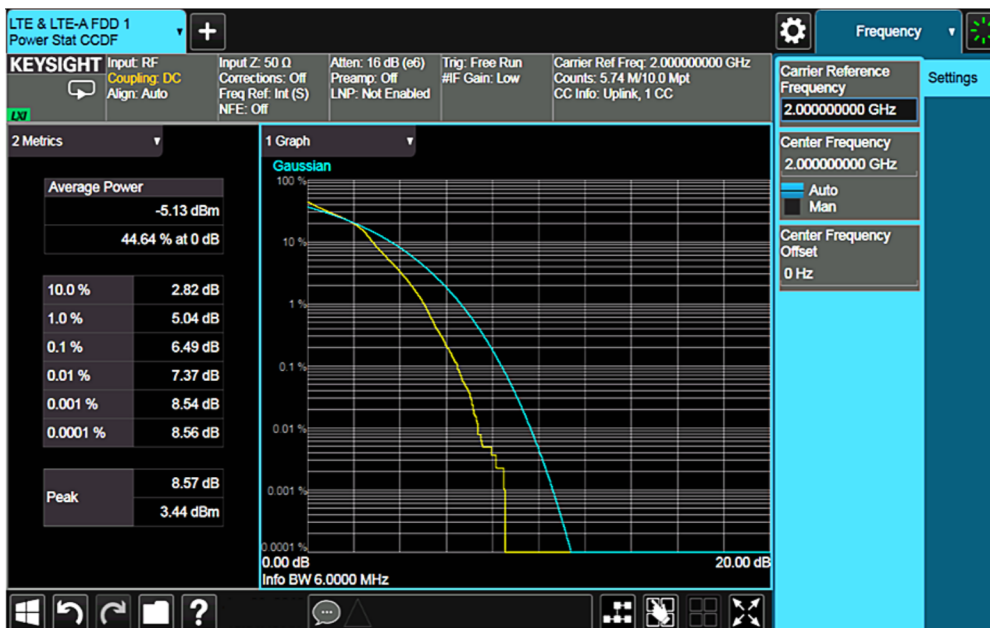
Figure 8-1. CCDF measurement
