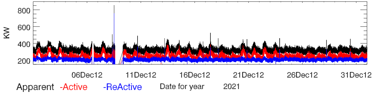
Site power data for dec2021. Power
