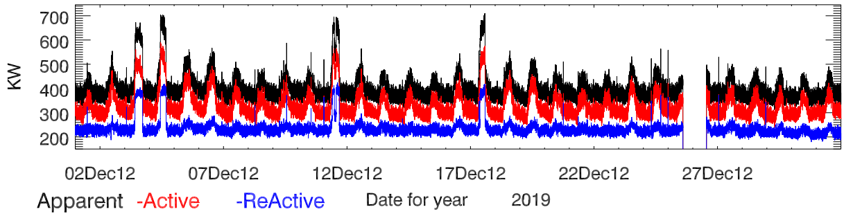
Site power data for dec2019. Power
