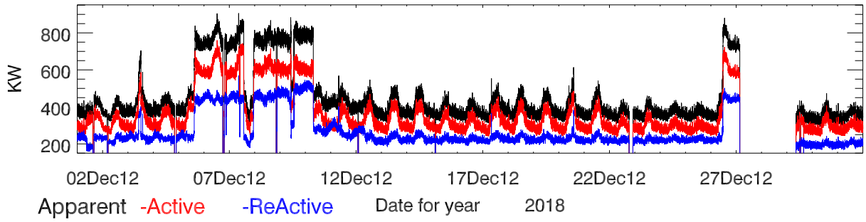
Site power data for dec2018. Power
