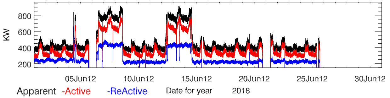
Site power data for jun2018. Power
