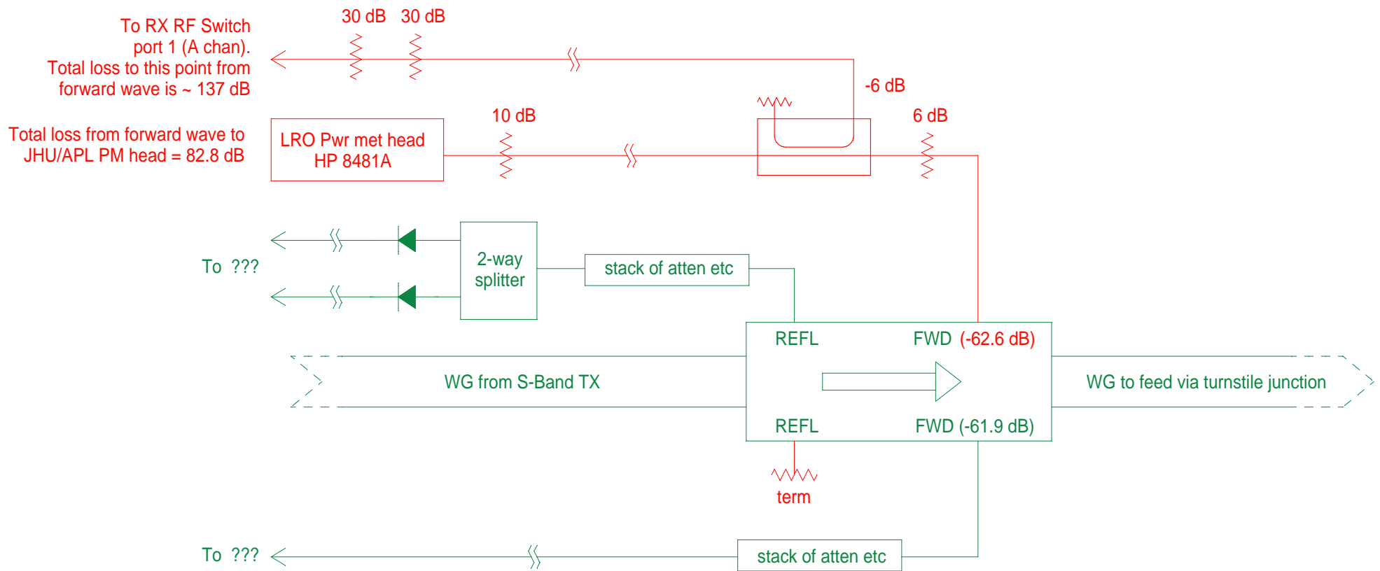
LRO-related changes to S-band monitoring system in dome as of 17 Nov 2011 (new/changed shown in red)
