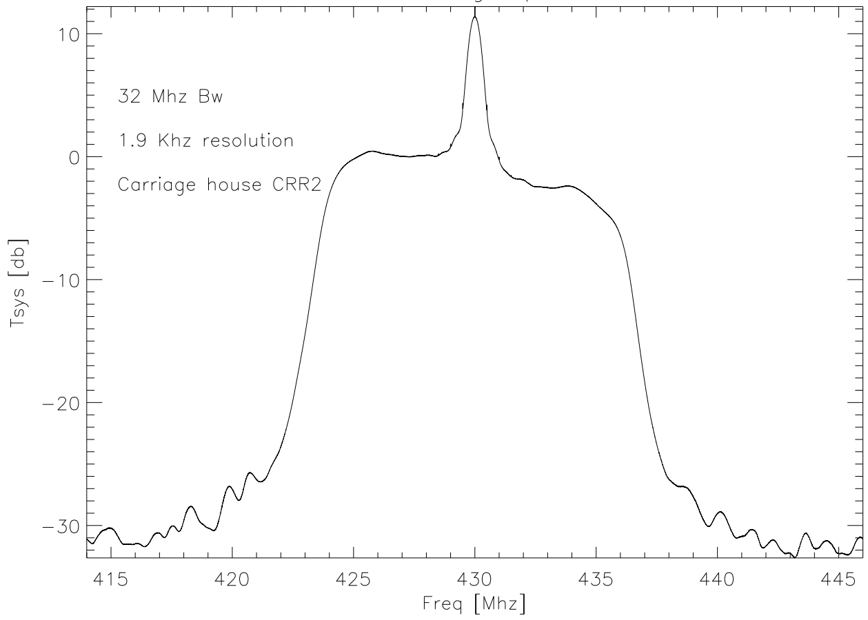
25oct09 rdev average spectra 10 secs.
