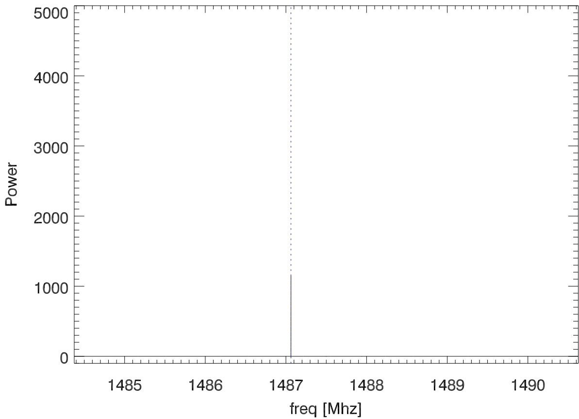
chan18 spectra (with image). 3.2 milliseconds of data
