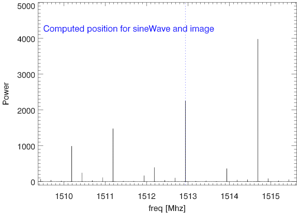
chan14 spectra (with sine wave). 3.2 milliseconds of data
