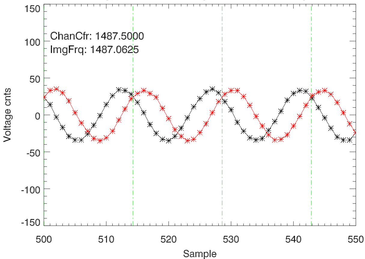
chan18 (gpu06,ch 2) Voltage vs sample. ImageChan
