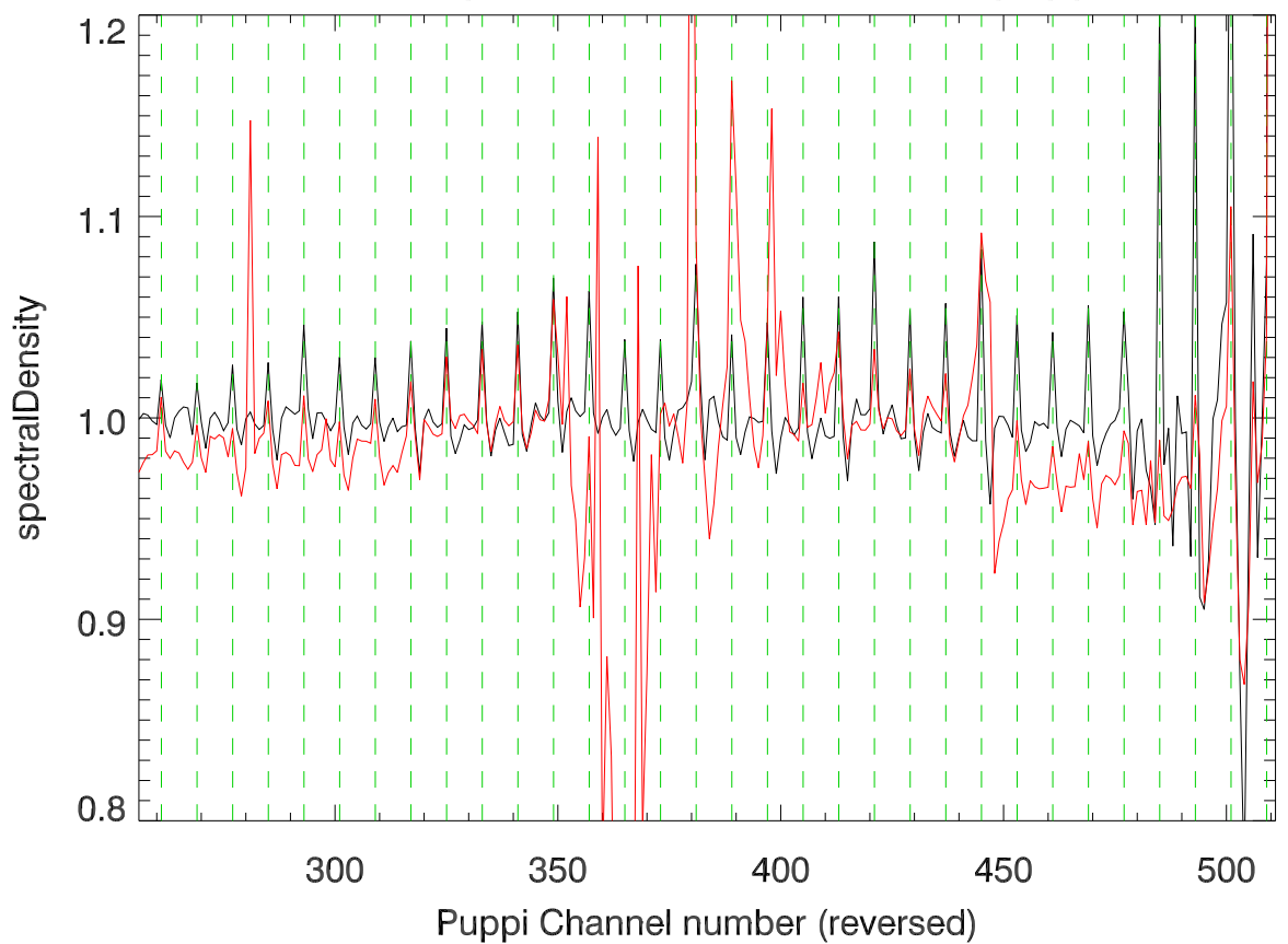
PoIB Comb overplot Cband,Lband SPC vs puppi channel
