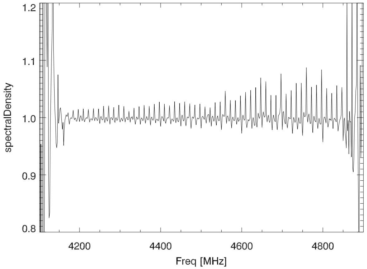
21apr18 P3054 bandPass corrected avgSpc (Cband) PoIB
