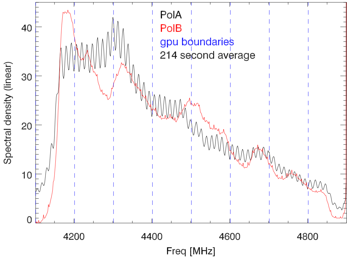
P3054 21apr18 AvgSpectra: puppi_58229_C0531+33_0289_0005.fits
