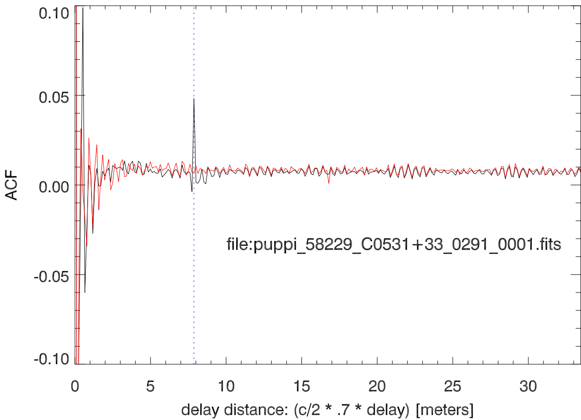
ACF of avg Lband spectra
