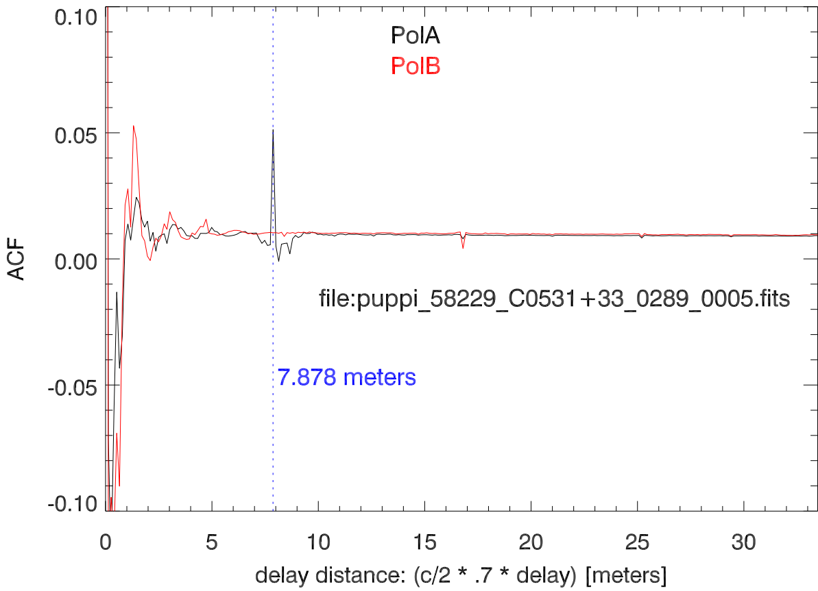
21apr18 P3054 ACF of avg Cband spectra
