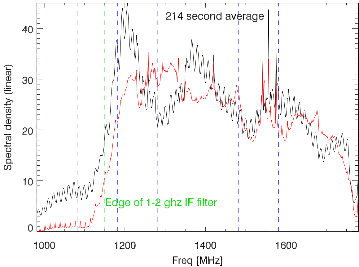
AvgSpectra.:puppi_58229_C0531+33_0291_0001.fits
