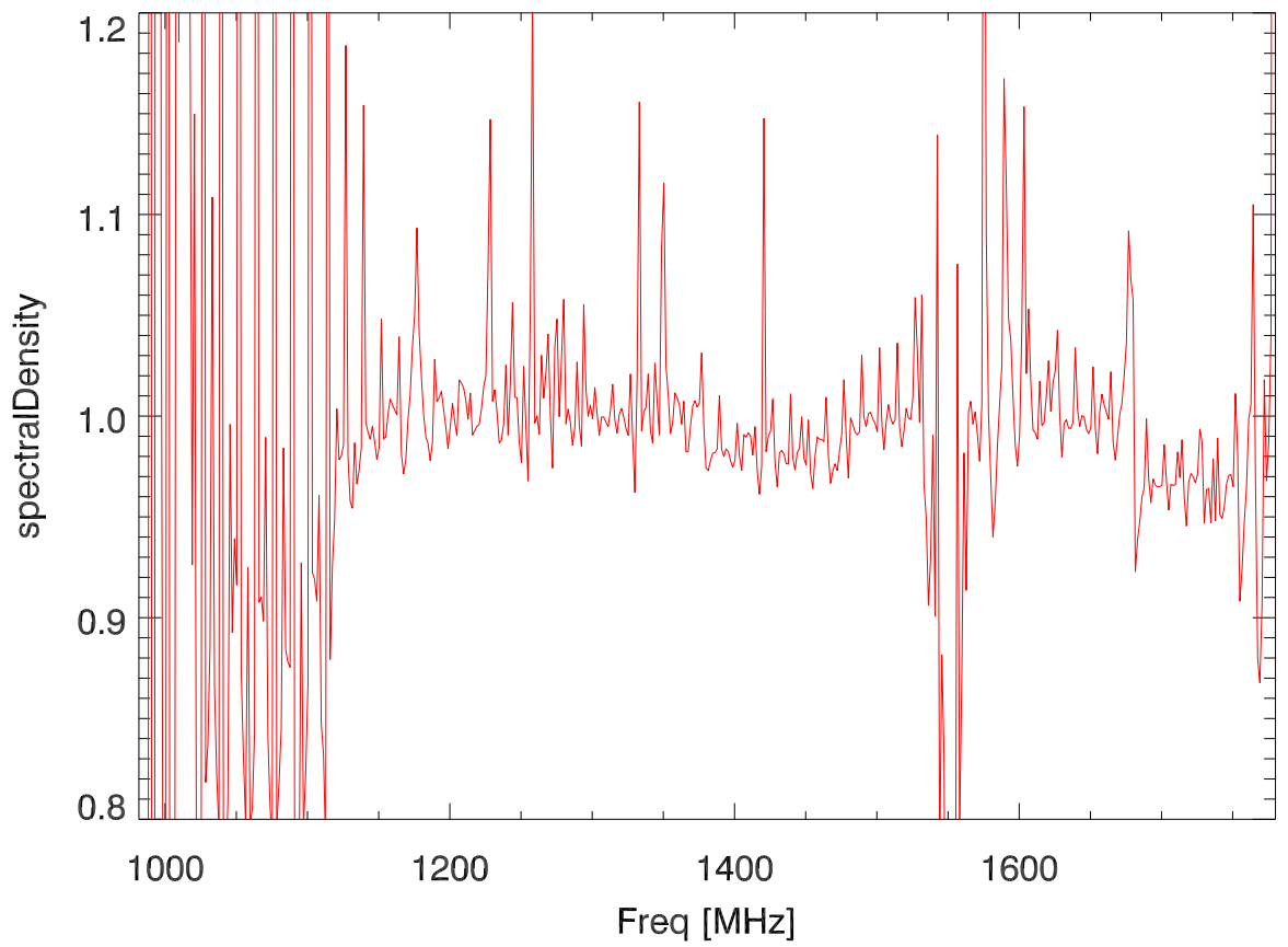
BandPass corrected avgSpc (Lband) PoIB
