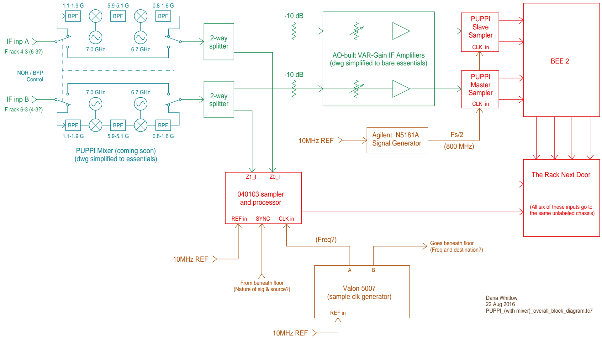
DANA'S REVISED ATTEMPT AT PUPPI SYSTEM BLOCK DIAGRAM
