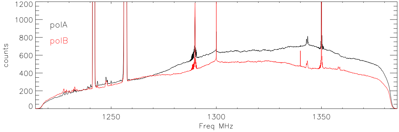
polA,B 1 second average spectra with offsets
