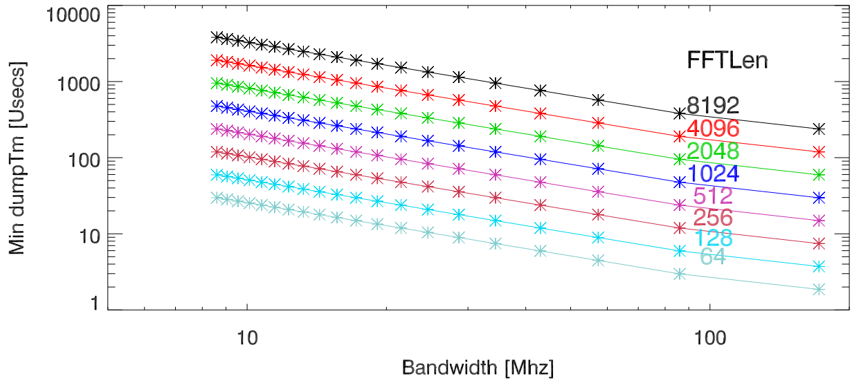
Mock Min dump times. SinglePixel. (Sum PoIS)
