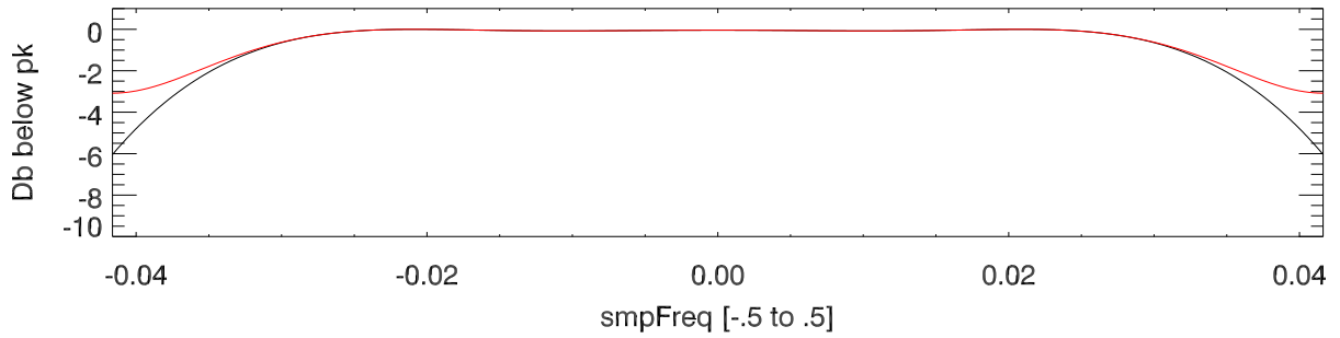
hanning
