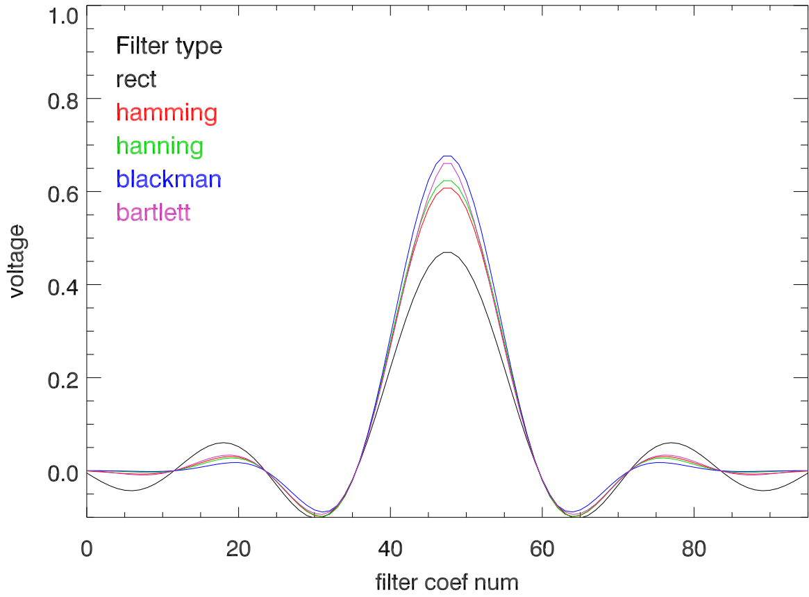
Time domain response Mock digFilt. dec= 12
