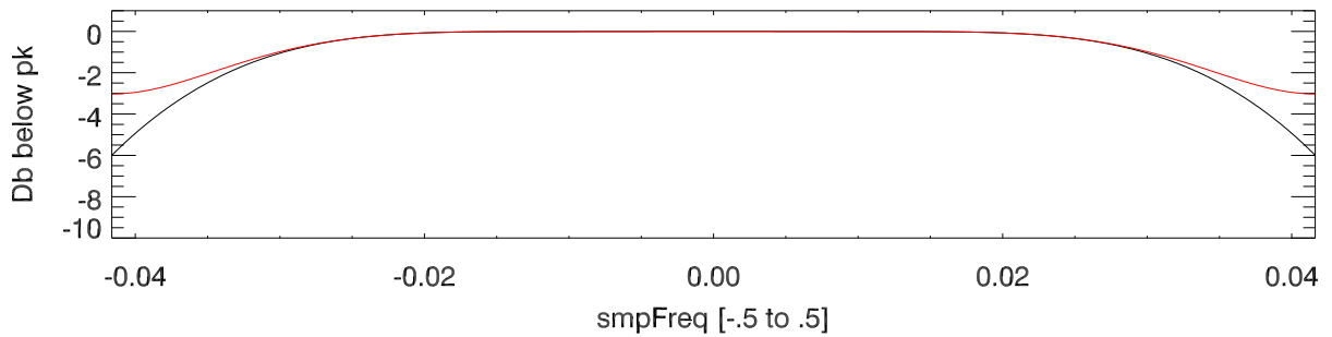
blackman
