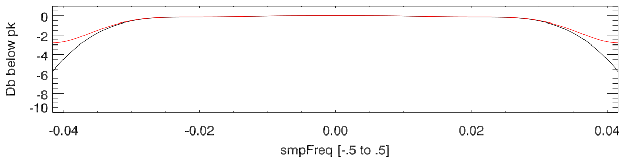
bartlett
