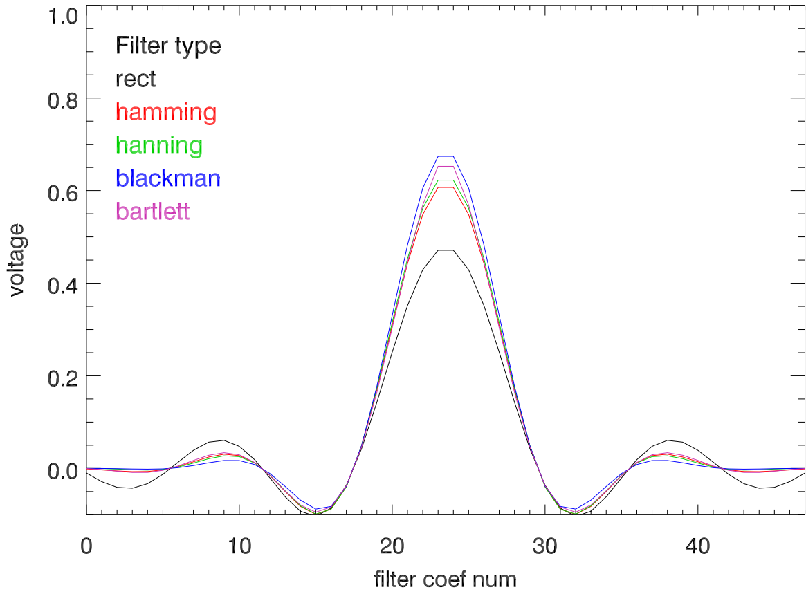
Time domain response Mock digFilt. dec= 6
