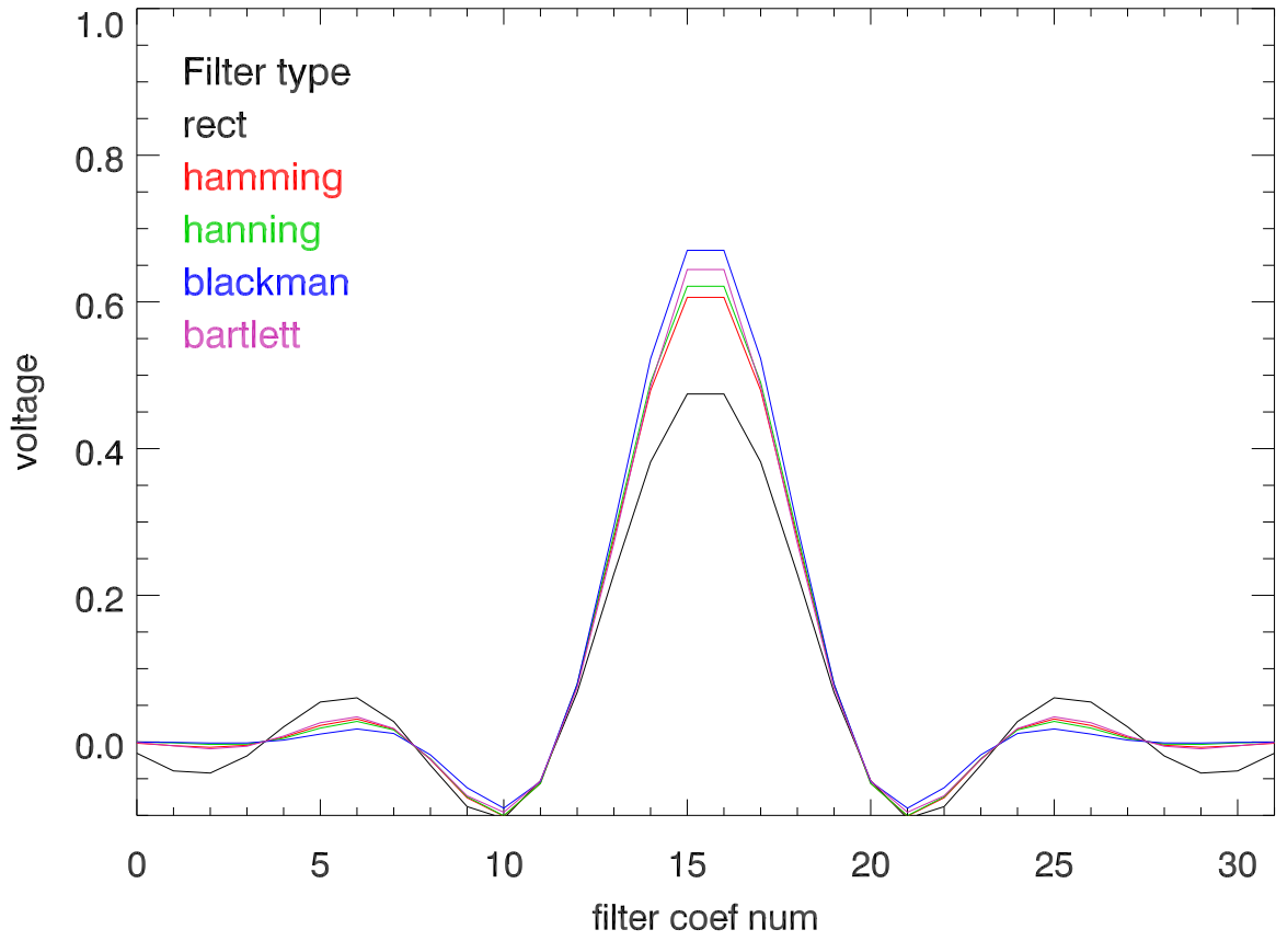
Time domain response Mock digFilt. dec= 4
