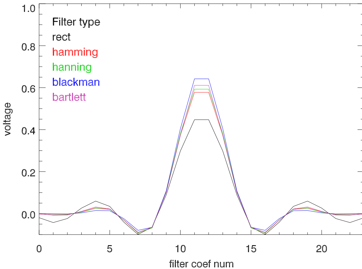
Time domain response Mock digFilt. dec= 3
