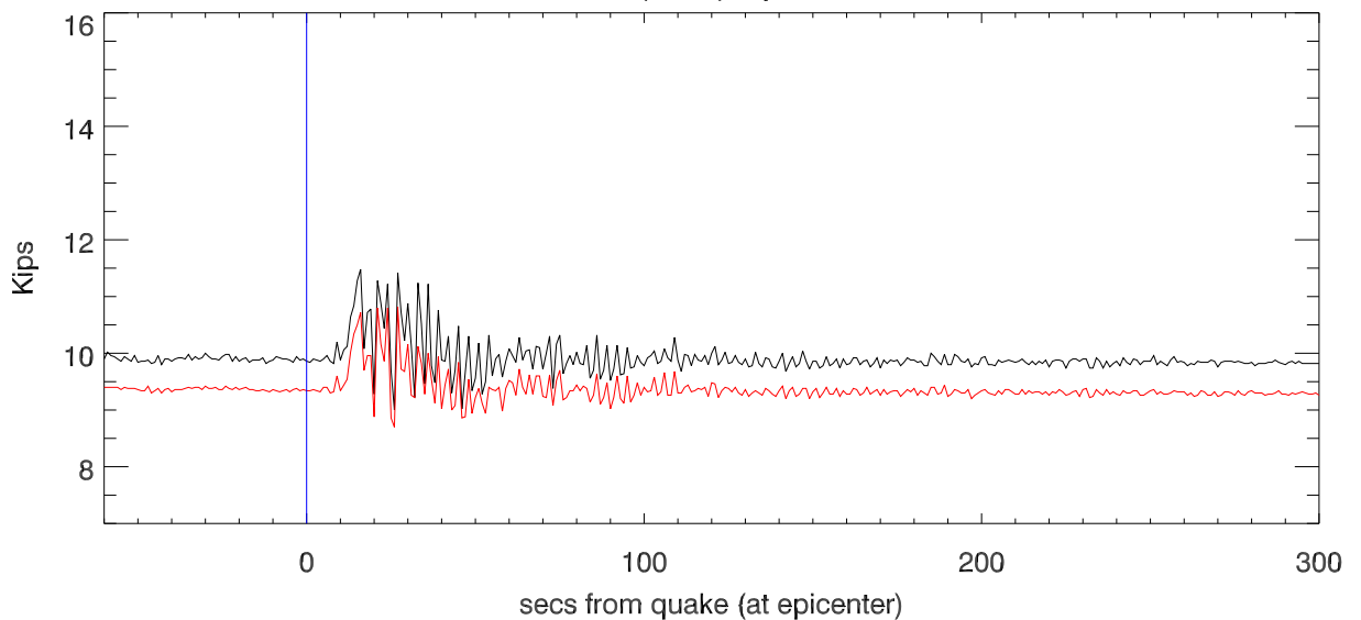
20200107 11:18:43(UTC) quake. tension in Td8
