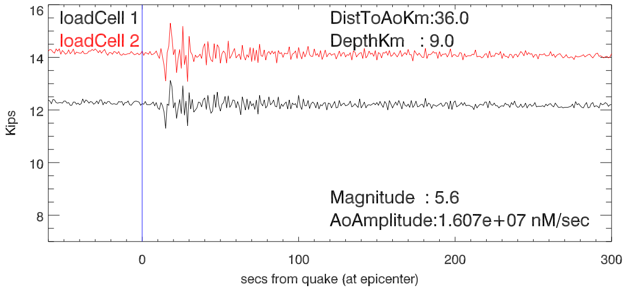
20200107 11:18:43(UTC) quake. tension in Td12
