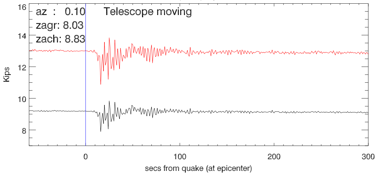
20200107 11:18:43(UTC) quake. tension in Td4
