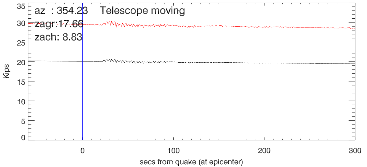
20200106 10:32:18(UTC) quake. tension in Td4
