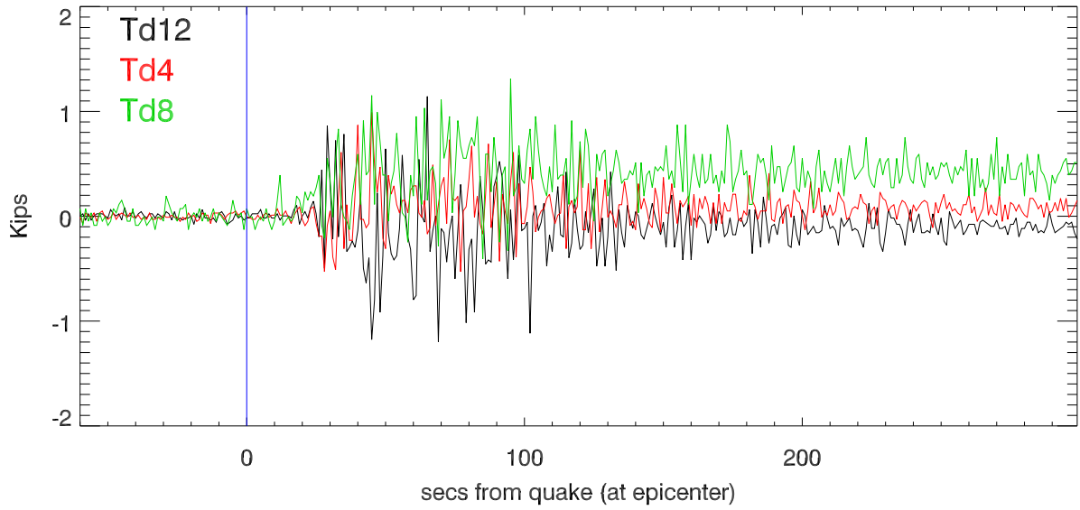
Kips change at each td corner vs time from epicenter
