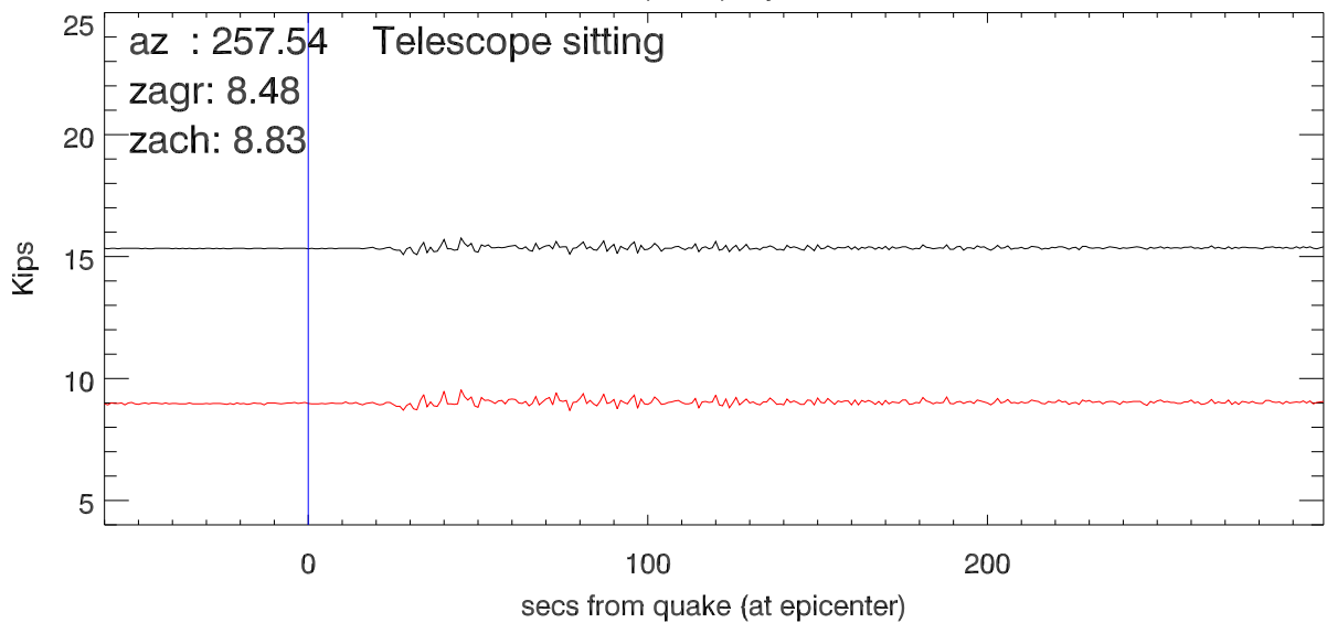
20190924 03:23:40(UTC) quake. tension in Td4
