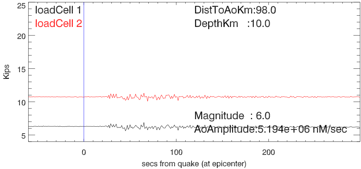
20190924 03:23:40(UTC) quake. tension in Td12
