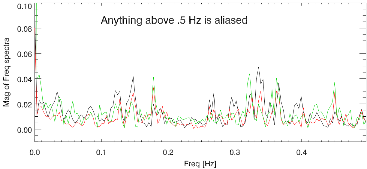
Magnitude of freq spectra around earthquake (for 3 tiedowns)
