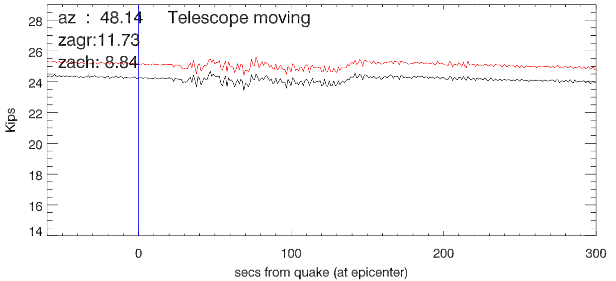
20140113 04:01:04(UTC) quake. tension in Td4
