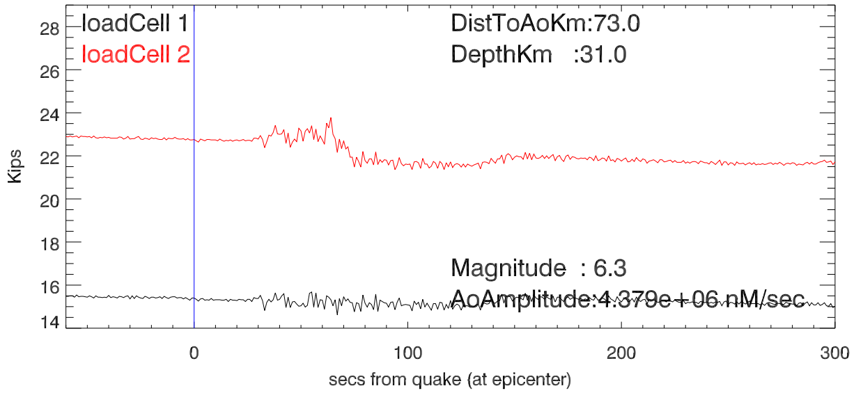
20140113 04:01:04(UTC) quake. tension in Td12
