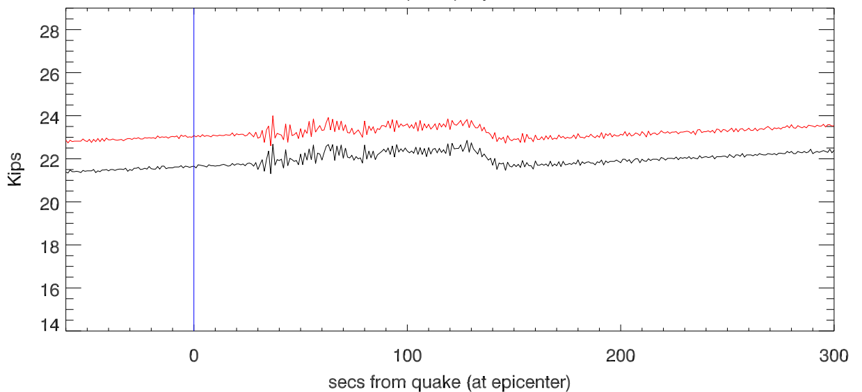
20140113 04:01:04(UTC) quake. tension in Td8
