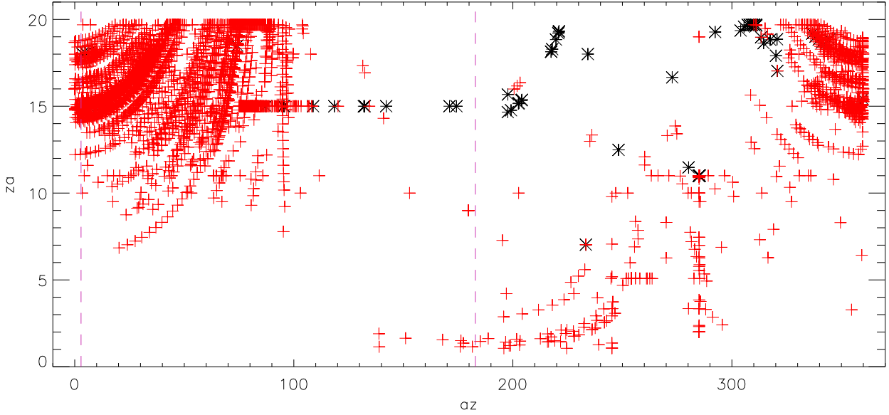
jan 2016 distomats 2,3 failures (T4) * DIST2 + DIST3
